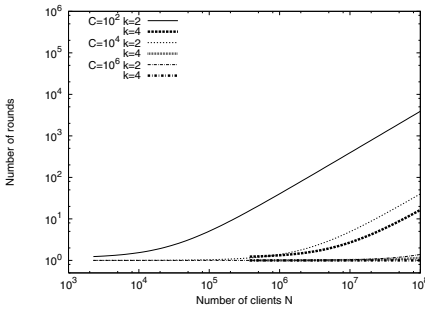
Fig. 8. Download time of the mesh architecture for different values of C ( k = 2 , s = 4 )
