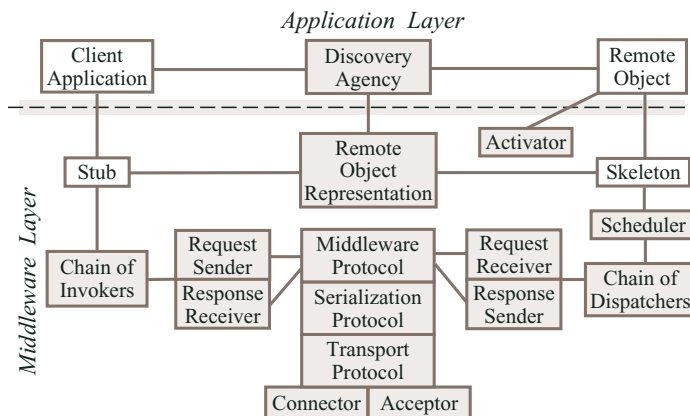
Fig. 1. Arcademis Architecture
