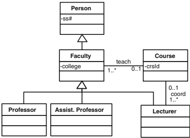
Fig. 3. Specialization Hierarchy
