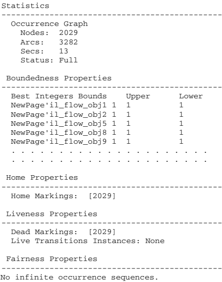
Fig. 7. The state space analysis standard report for the CP-net of Figure 6
