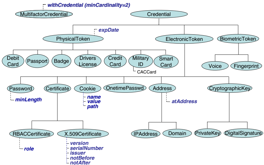
Fig. 4. Credentials Ontology
