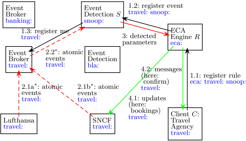
Fig. 7. Language-Centered Communication
