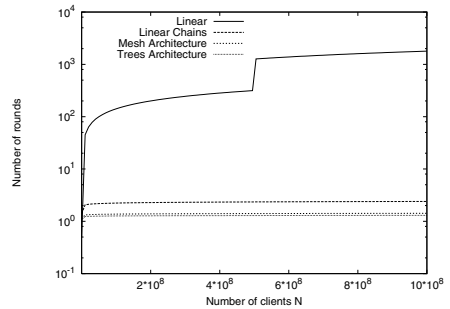
Fig. 13. Download time for different architectures with k = 4 , C = 100 and s = s_{max} . Linear shows the completion times for a population of 10^9 peers with symmetric bandwidth.
