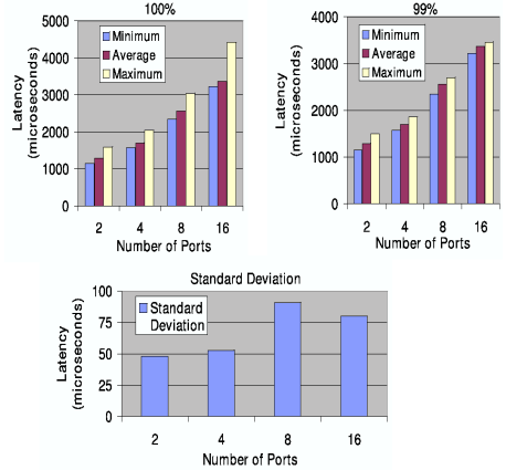
Fig. 9. Latency Measurements for Reconnecting Component Connections
