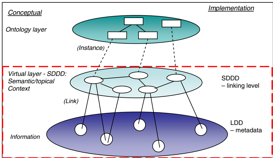
Fig. 2. Layered solution
