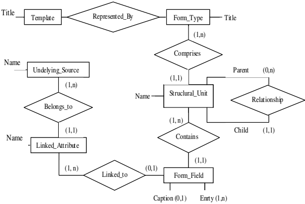
Fig. 1. Form Model
