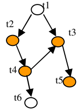
Fig. 1. Blocker Chain
