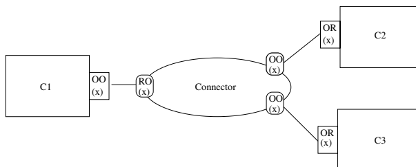
Fig. 4. A connector
