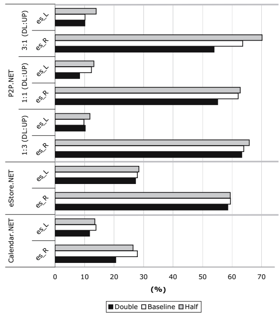
Fig. 3. Effect of Heap Size on the Survival Ratio
