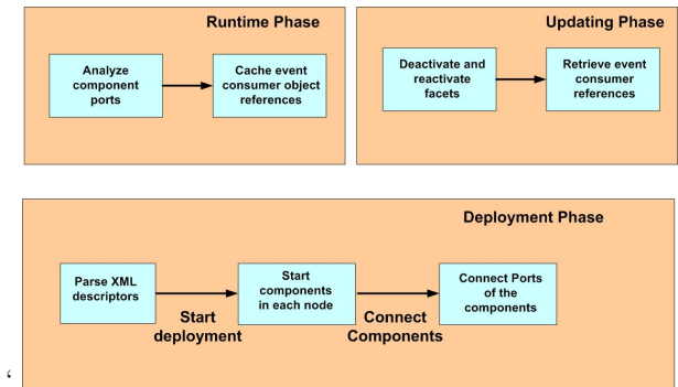
Fig. 5. Enabling (Re)connections of Components in SwapCIAO
