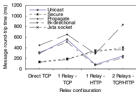
Fig. 9. Effects of relay configurations on pipe RTT
