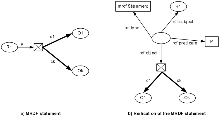
Fig. 7. Reification in Multidimensional RDF
