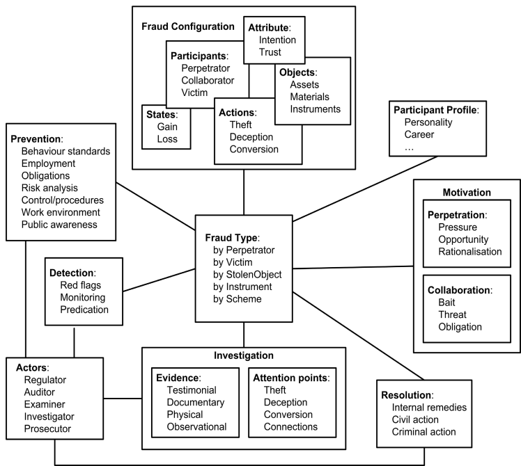
Fig. 4. Architecture of the fraud ontology
