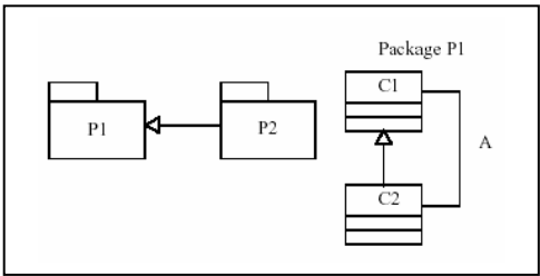
Fig. 2. Example of a MOF metamodel
