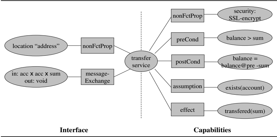
Fig. 4. Ontological Service Template (WSMO)
