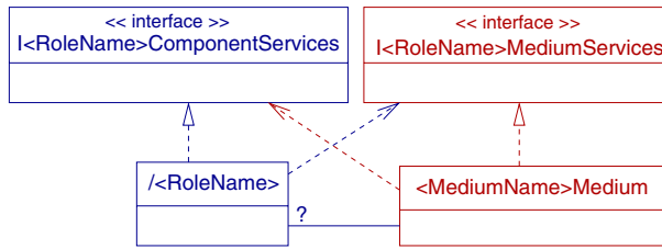
Fig. 5. Generic UML model of a communication component
