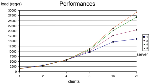
Fig. 8. Load Balancing performance (request per second)
