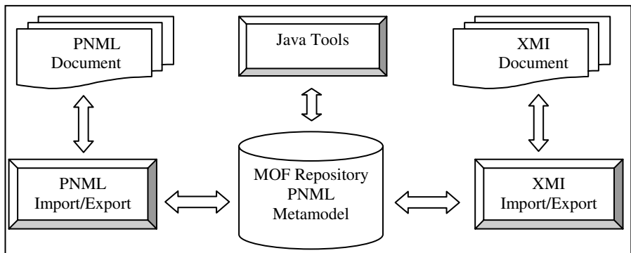
Fig. 6. Architecture of PNML and XMI documents Import/Export Modules
