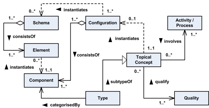
Fig. 2. A design pattern in UML for the architecture of topical ontology
